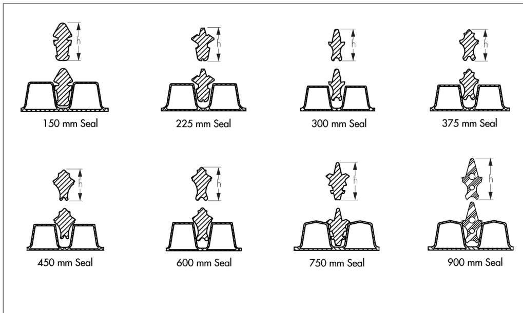
Figure 4 Twinwall seal dimensions
