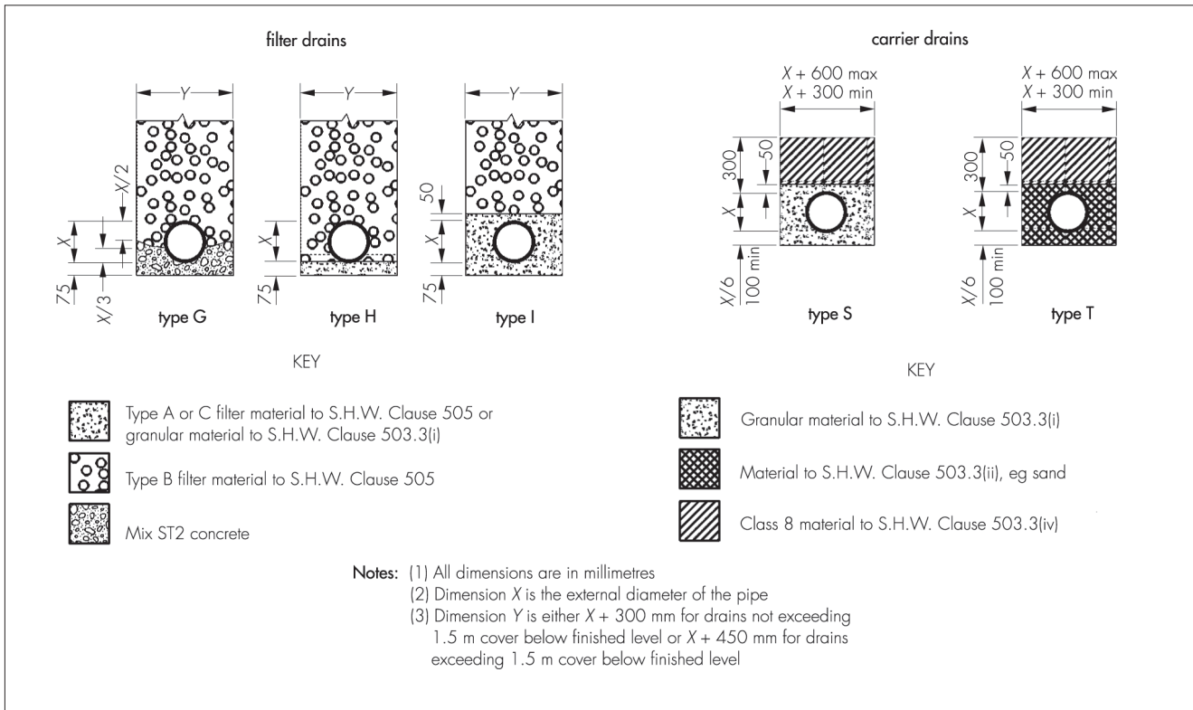
Figure 5 Installation details
